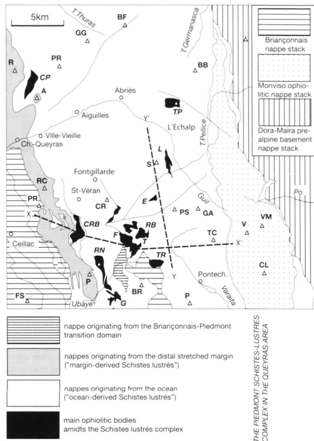
Fig. 2. Structural sketch-map of the Queyras area and its surroundings (modified after Tricart et al. 2003). Main peaks and summits: A: Arenier; BB: Bric Bouchet; BF: Bric Froid; BR: Bric de Rubren; CL: Cima delle Lobbie; CR: Château-Renard; FS: Font-Sainte; GA: Grande Aiguillette; GG: Grand Glaiza; P: Pérouv; PR: Pointe de Rasis; R: Rochebrune; RC: Roche des Clots; S: Ségure; TC: Tre Chiosis; V: Viso; VM: Viso Mozzo. Main ophiolitic bodies: CRB: Cascavelier-Rocher Blanc; E: Eychassier; F: Farnéiré; G: La Gavie; L: La Lauze; CP: Col de Péas; RB: Rocca Bianca; RN: Roche Noire; T: Tête des Toillies; TP: Tête du Pelvas; TR: Tour Real. XX' orogen-perpendicular section and YY' orogen-parallel section of Plate 1.
