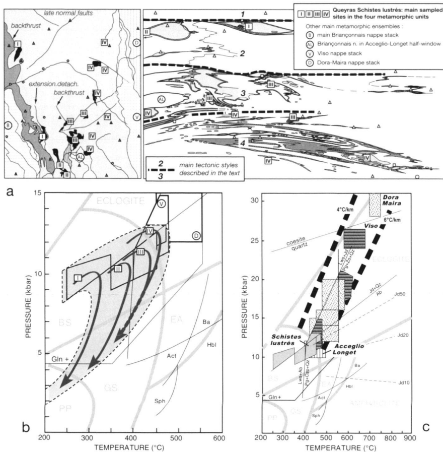
Fig. 6. The four main blueschist-bearing early-formed units of Queyras Schistes lustrés in their regional metamorphic context. a: Sketch map (see Fig. 2) and N-S section (see YY' in Plate 1) with location of the main sampled ophiolites. 1 to 4: main tectonic styles described in the text. b: The main metamorphic assemblages observed in the mafic rocks and their P-T conditions of formation and retromorphic evolution. The eclogitic conditions in the Viso ophiolites (Schwartz et al. 2000a) and the Dora-Maira massif (Michard et al. 1993) are indicated for comparison. Metamorphic facies is from Spear (1993) with: PP, prehnite-pumpellyite; GS, greenschist; BS, blueschist; EA, epidote amphibolite; AM, amphibolite. The stability of glaucophane (Maresch 1977), lawsonite (Heinrich & Althaus 1988), coesite (Bohlen & Boettcher 1982), titanite (Moody et al. 1983) and calcosodic-amphibole (Ernst 1979), the reaction Jd+Qz = Ab (Holland 1980) and the jadeite isopleths (Gasparik & Lindsley 1980) are indicated. c: Compilation of HP-LT conditions available along the same Alpine transect in the Queyras – Viso units (Nisio & Lardeaux 1987; Messiga et al. 1999; Schwartz et al. 2000a) and the Dora-Maira units (Chopin et al. 1991; Michard et al. 1993).
