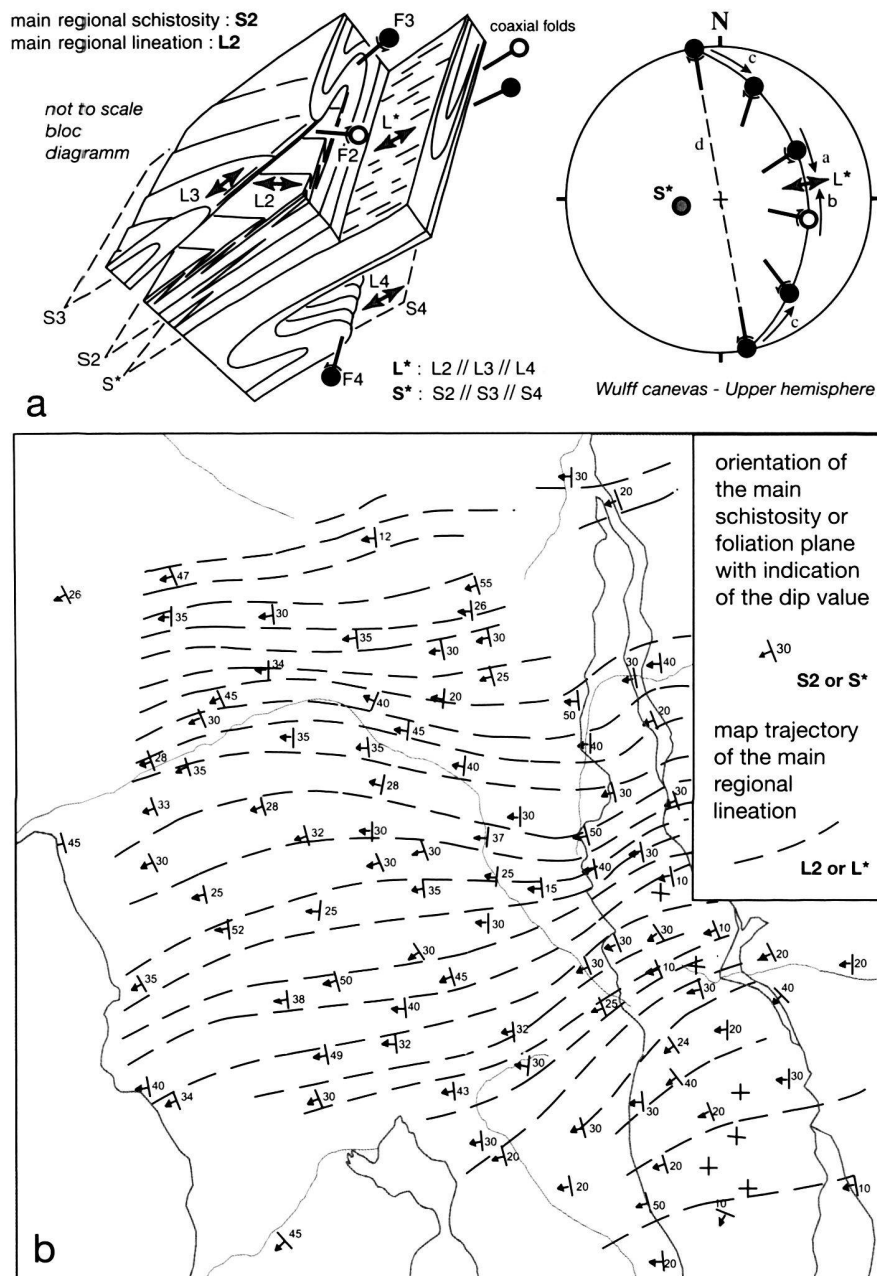
Fig. 4. The isoclinal structure of the Queyras Schistes lustrés. a: synthetic block diagram and stereonet showing the geometrical relationships between the folds (F), schistositys (S) and lineations (L) associated with the successive D2, D3 and D4 deformation phases. For clarity, the original flat-lying S1 foliation and the associated F1 isoclinal folds have been omitted (see "sandwiched marbles" in section YY', Plate 1). As proposed by Hansen (1971), arrows turning around the fold axis symbols indicate the asymmetry patterns of folds in terms of rotation of short limbs relative to long limbs about their hinge lines, the folds being observed down-plunge of the hinge line. The double grey arrows recall the importance of stretching along the successive generations of lineations. The L2 lineation is deformed around the hinge of a F3 fold. Just below, in a zone of accentuated D4 deformation, the earlier formed schistositys become parallel to S4, resulting in a single planar structure S*. The earlier formed stretching L2 and L3 lineations rotate within this plane S* and become parallel to the L4 stretching lineation, resulting in a single very strong stretching lineation L* of composite origin. After a comparable rotation (arrows a and b in the stereonet), the axes of the F2 and F3 folds also become parallel to L* (coaxial folds). Another consequence (not represented in the block diagram) is that the axes of the F4 folds, dominantly small-scale folds, leave their initial N-S horizontal orientation and start rotating (arrows c in the stereonet) within S4 toward the L4 direction of stretching, resulting in axes with a planar dispersion and hinges with a non-cylindrical geometry. In the stereonet, the dashed line (d) represents the projection of the plane of the section YY' (Plate 1). b: regional orientation of the dominant schistosity and lineation (same structural sketch map as in Fig. 2).
