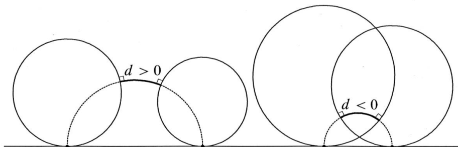
FIGURE 4 The signed distance of horocycles
