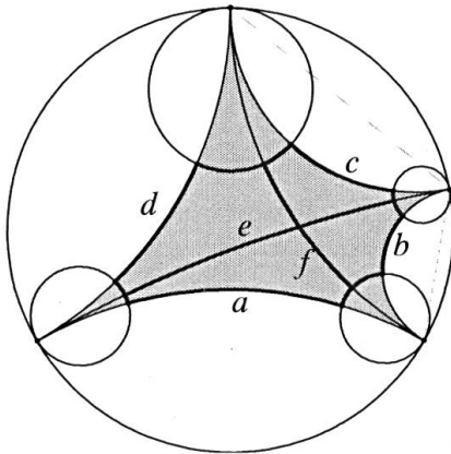
FIGURE 11 Ptolemy relation
