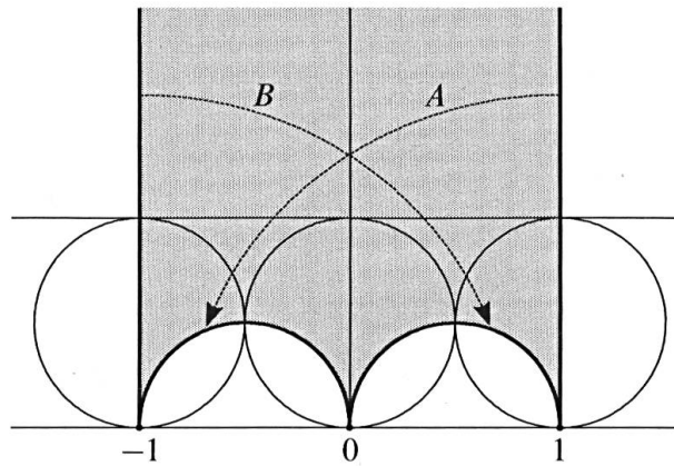
FIGURE 13 The modular torus
