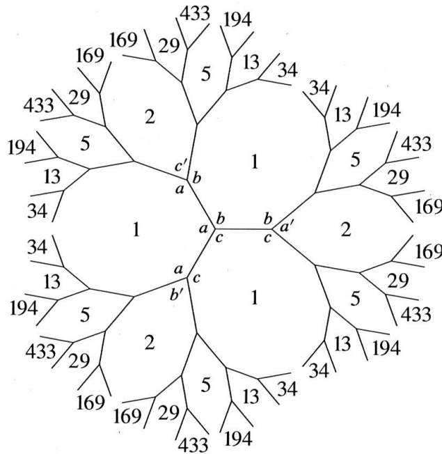
FIGURE 1 Markov tree
