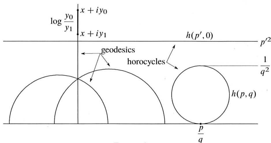
FIGURE 2 Geodesics and horocycles
