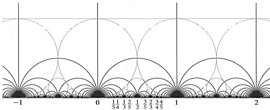
FIGURE 6 Ford circles and Farey tessellation
