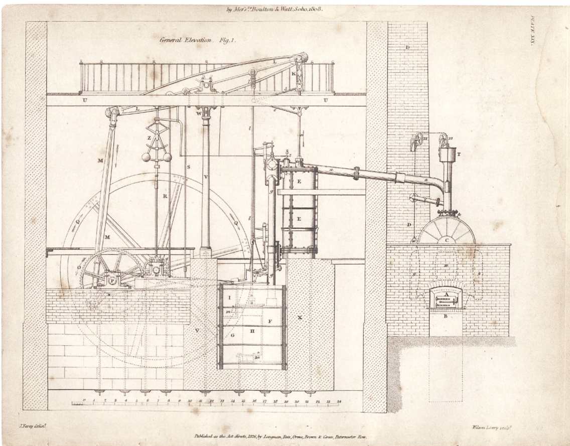
3 Top: Boulton & Watt steam engine of 10 HP, produced from about 1787 to 1800.
