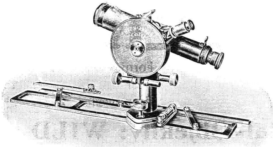
Kippregel No. 76
