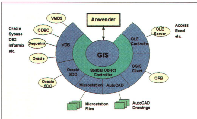
Abb. 1: SMALLWORLD Open-Client-Architektur.
