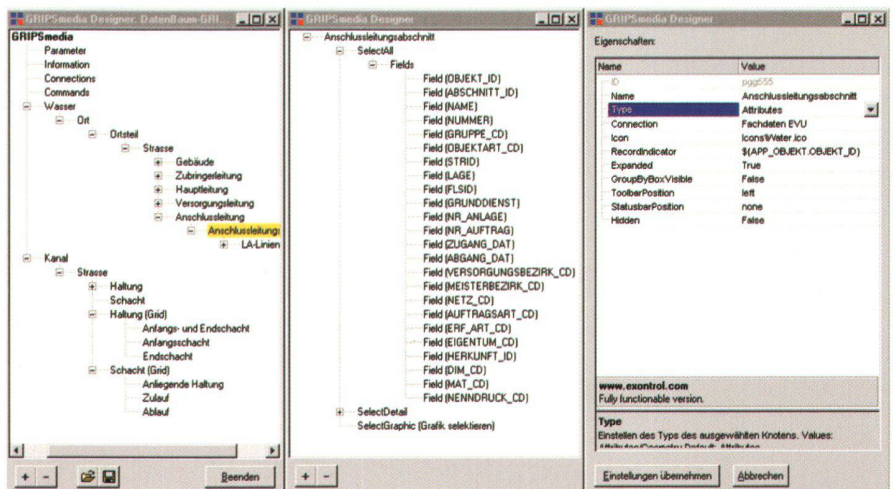
Abb. 15: GRIPSMedia Designer.
