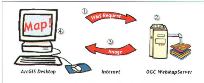
WMS-ArcGIS-Prinzip.
