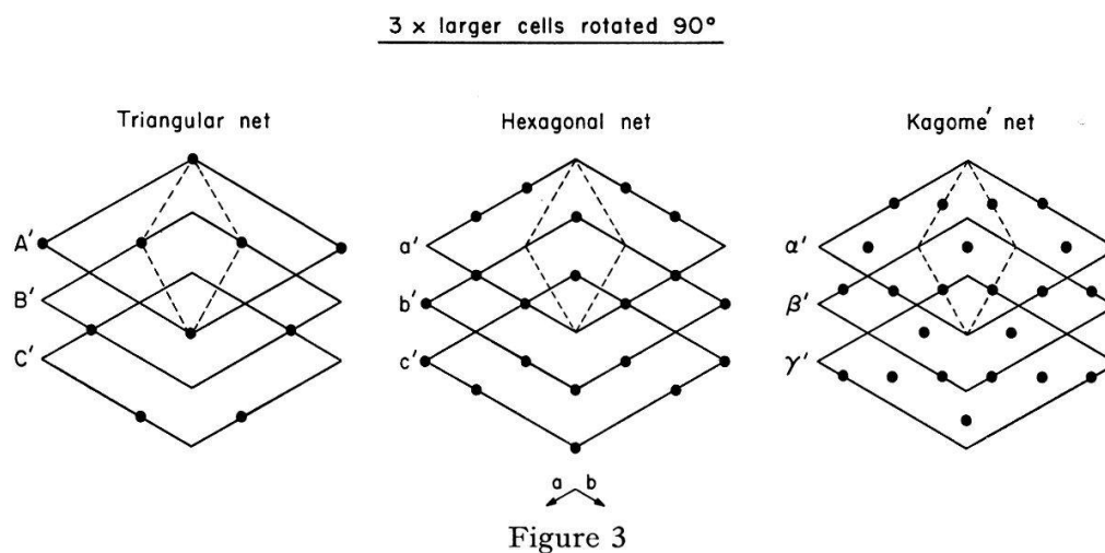
Triangular, hexagonal and kagomé nets of atoms in three stacking positions ( A', B', C'; a', b', c'; \alpha', \beta', \gamma' respectively) relative to a basal hexagonal cell which contains respectively 3, 6 and 9 atoms per net.
