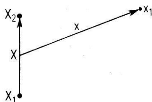
Figure 1 Jacobi coordinates.
