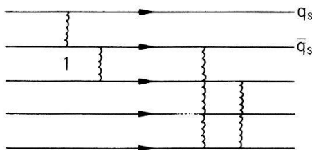
Figure 9 The view of a baryon if q\bar{q} pairs are important for all x .
