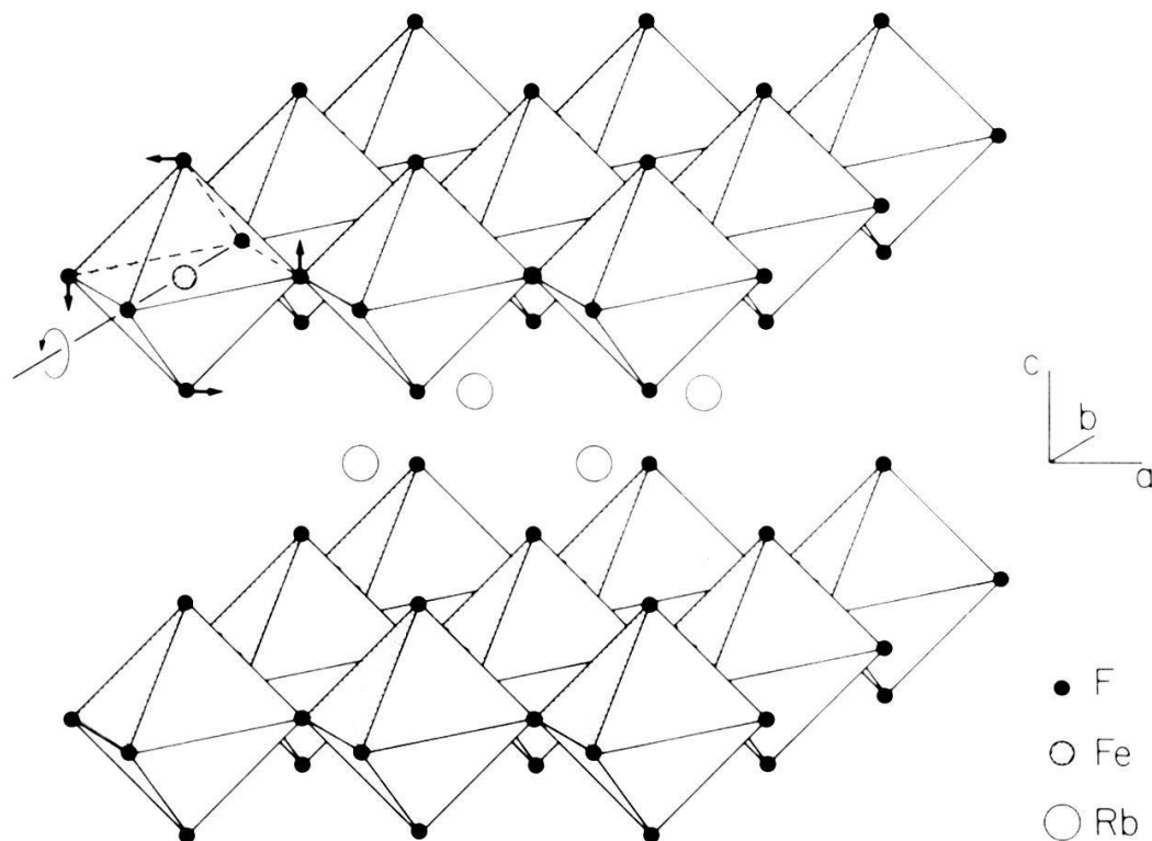
Figure 1 Idealized crystal structure of \text{RbFeF}_4 . The \text{FeF}_6 octahedra are shown without distortion or tilting. The arrows indicate the rotations of the octahedra in phase II.
