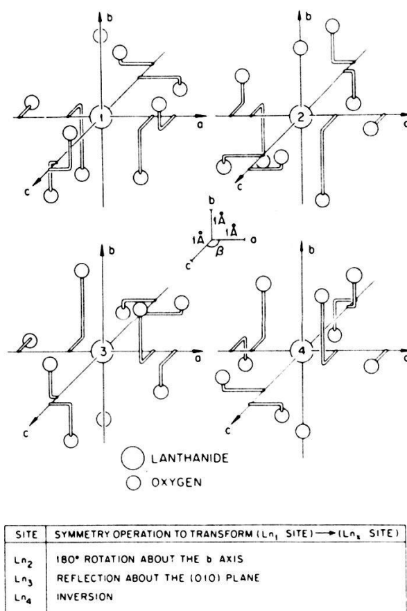
Fig. 7. Position of the 9 nearest-neighbours O ions surrounding the 4 rare-earth sites in the unit cell of monazite. The symmetries which transform site 1 into the three others are listed below.
