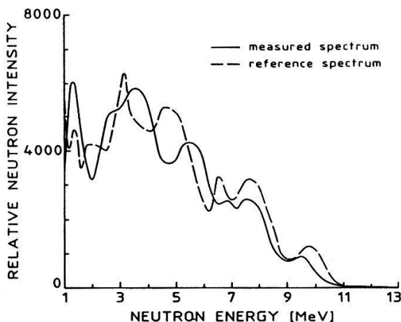
Fig.1: unfolded spectrum PuBe source with NE-230 spectrometer
