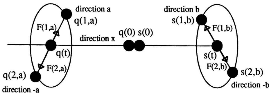
The system of two particles q and s that move outwards on a rigid rod in direction x , together with the measuring apparatuses, that consists of diametrically located particles q(1, a) and q(2, a) on a circle A at the left in a plane orthogonal to x , and diametrically located particles s(1, b) and s(2, b) on a circle B at the right, in a plane orthogonal to x (fig 6).
