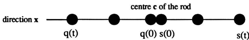
The system of two particles q and s bounded on a rigid rod in direction x , that move outwards, q to the left and s to the right (fig 5).
