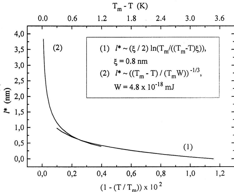
Fig. 3. Layer thickness vs. 1-T/T_m . The increase in thickness is determined by a logarithmic growth for T_m-T > 0.5\text{K} with a correlation length \xi = 0.8\text{nm} and by a power law growth for T_m-T < 0.2\text{K} with a Hamaker constant W=4.8\times 10^{-18}\text{mJ} . The cross-over thickness is comparable with the correlation length in the layer: l_c^*=(0.7\pm 0.1)\text{nm} .
