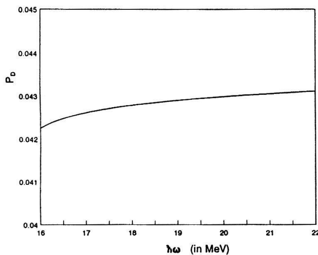
Fig.6 Variation of The Deuteron D-state probability with \hbar\omega
