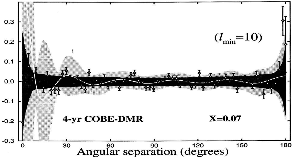
Figure 1: The collapsed three-point function (white curve) and the rms cosmic variance (grey band) which includes also the \sim 50\% increment due to the sample variance, in units of 10^4 \mu\text{K}^3 , as predicted by the analytical texture model. The asymmetry parameter is x = 0.07 , as suggested by simulations. Also shown is the ‘pseudo-collapsed’ three-point function as computed from the analysis of the four-year COBE-DMR data. Error bars represent instrument noise while the dark band represents the rms range of fluctuations due to a superposition of instrument noise and cosmic and sample variance.
