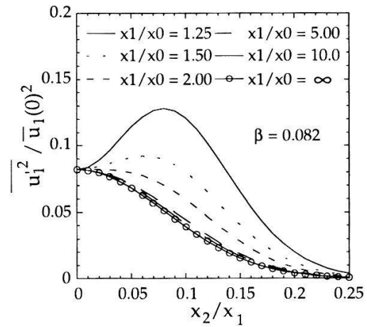
Figure 2: The normal Reynolds stress for different distances x_1/x_0 . The quantity x_0 denotes the core distance of the jet.
