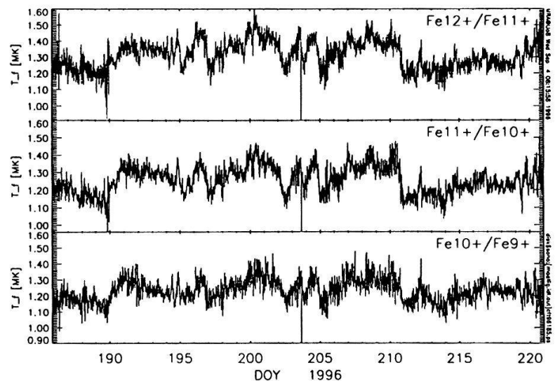
Fig. 1: Iron freeze-in temperatures.
