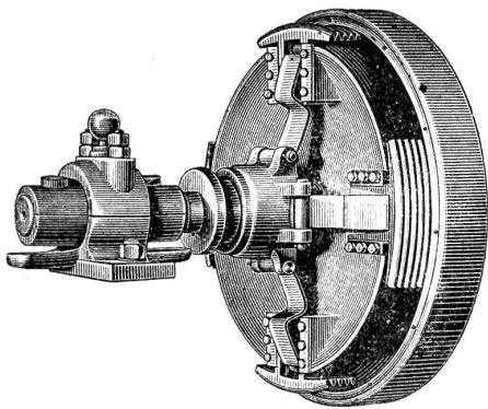
Frictionskupplung
