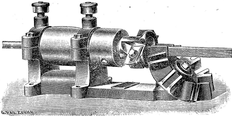
Rundstabhobelmaschine
