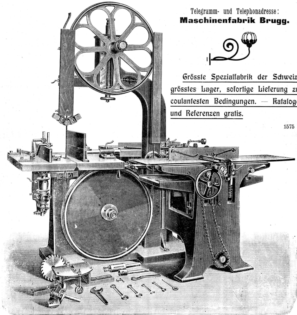
Universalmaschine No. 3.
