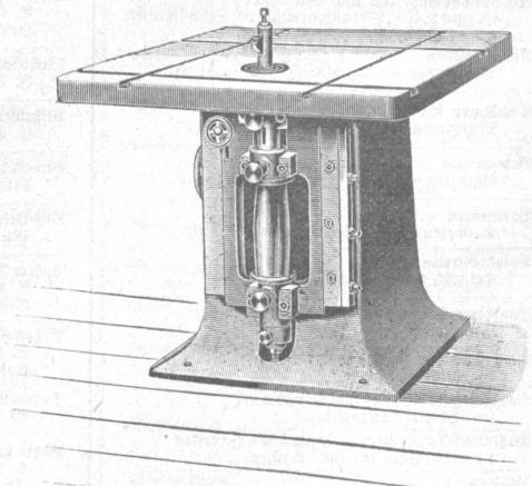
Kehlmaschine.
