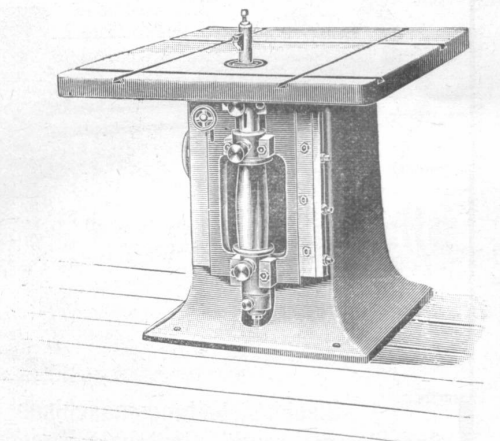
Kehlmaschine.
