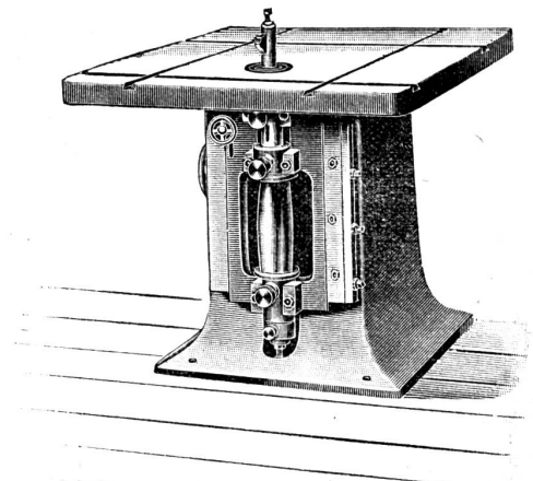
Kehlmaschine.
