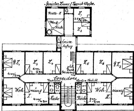
Dachstock.
