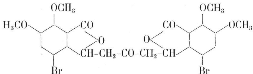
[ Di-(Brommekonin-)Aceton ]
