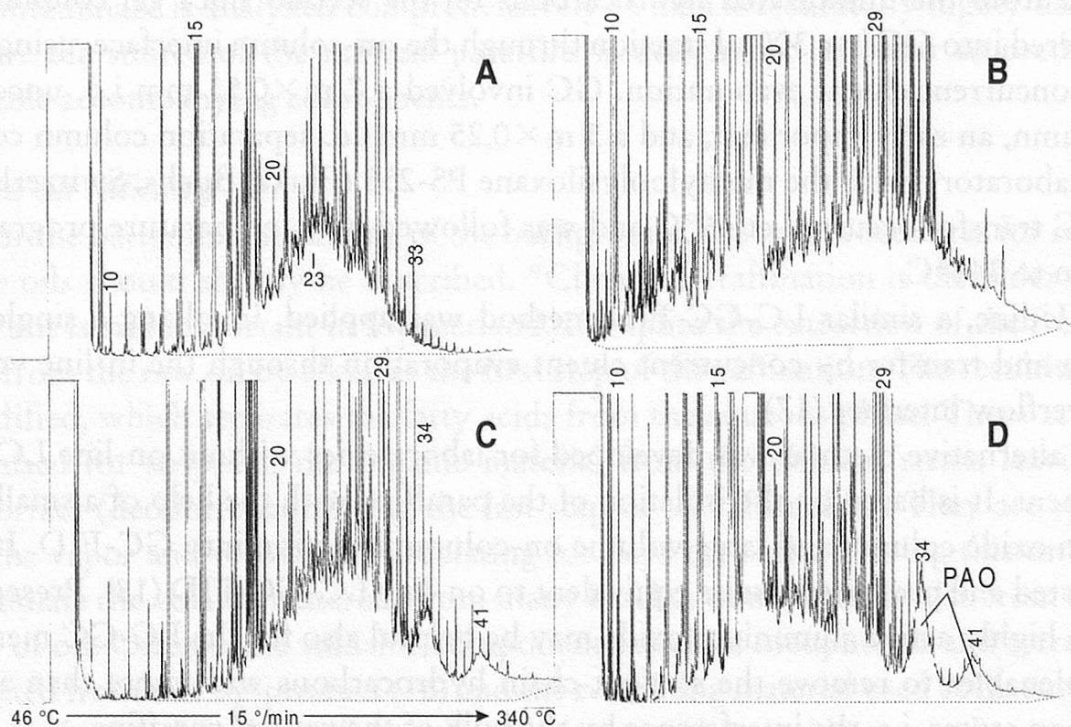
Figure 1 Examples of paraffins in the by-products from edible oil refining. PAO, poly alpha olefines
