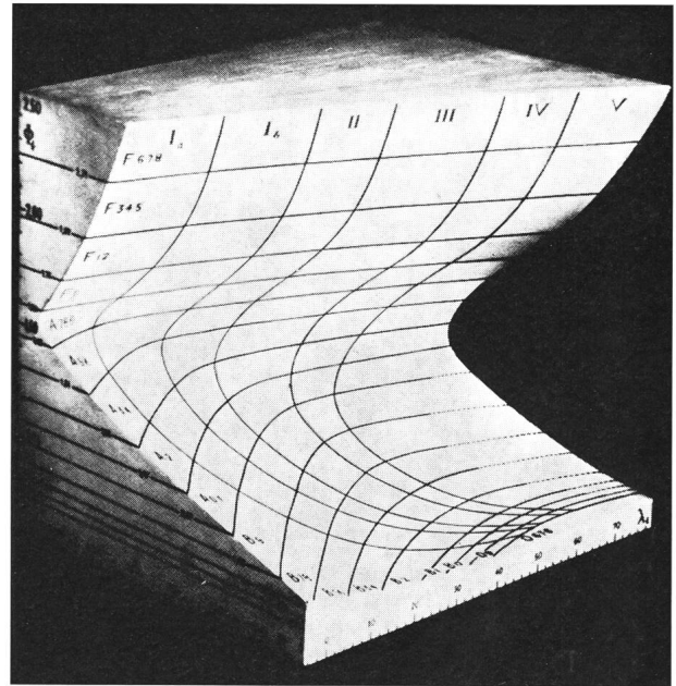
Fig. 2: Surface \Sigma .
