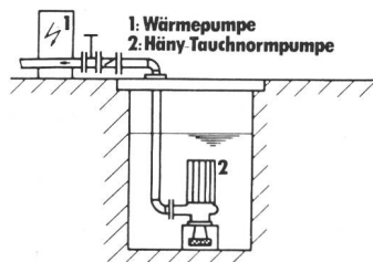
Tauchnormpumpe
