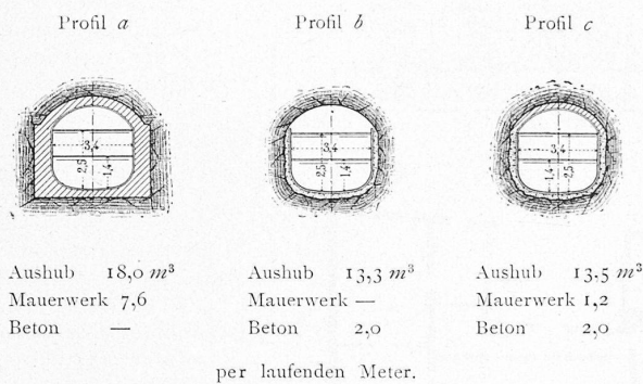
Fig. 5—7. Tunnel-Profile.
