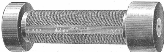
Toleranz-Kaliberdorn.
