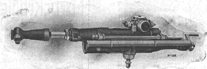
Schwere Tunnelbohrmaschine System Meyer D.R.P. — D.R.P. a.
