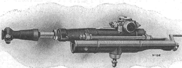
Schwere Tunnelbohrmaschine System Meyer D.R.P. — D.R.P. a.
