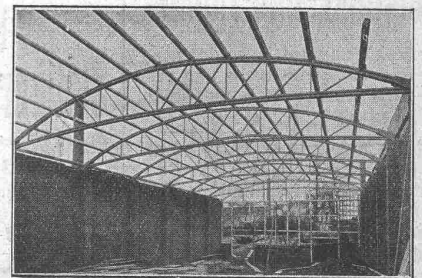
Dachbinder in Holz, System Meltzer.
