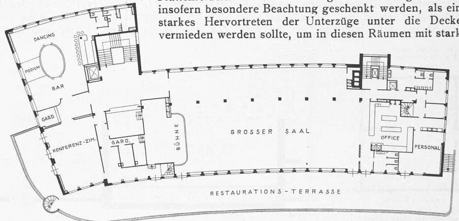
Abb. 19. II. Stock.
