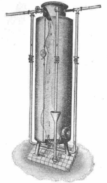
Magno-Filter
