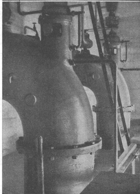
Vertikal-Propellerpumpe 30 000 lit/min
