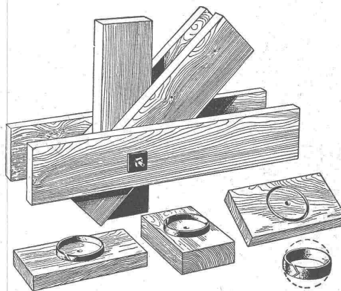
RINGDÜBEL + PATENT
