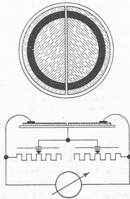
Bild 8. Differential-Photoelement
