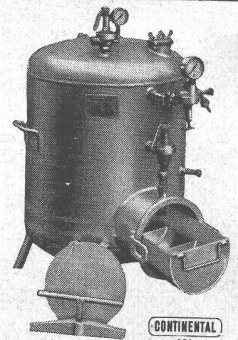
Acetylenapparate
