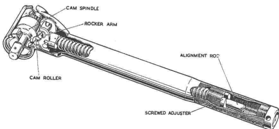
(c) "ACRATORCK" TYPE TORQUE WRENCH
