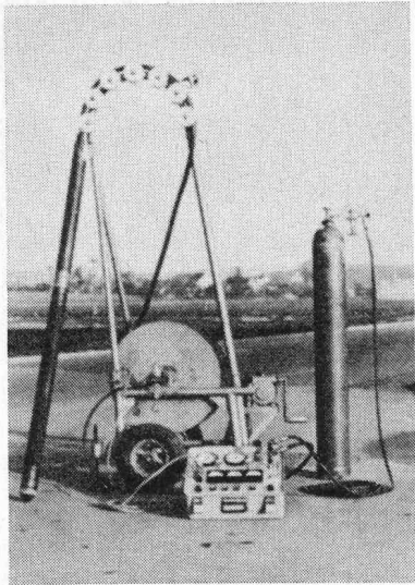
Dilatometer 95
