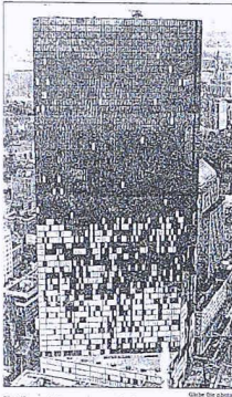
The Hancock Tower was speckled with p. wood in 1973 as engineers tried to figure out why its windows were cracking.
