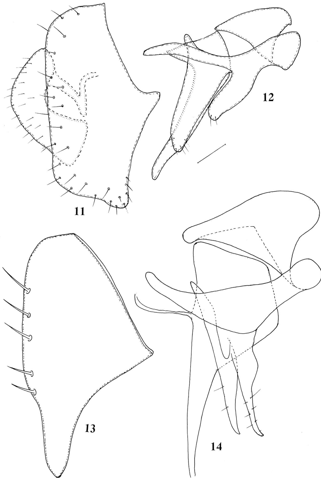
Figs 11–14. Figs 11–12: Parochthiphila nigripes (STROBL), ♂ genitalia, lateral view. 11, eandrium; 12, hypandrial complex. – Figs 13–14: Leucopis celsa TANASIJTSHUK, ♂ genitalia, lateral view. 13, eandrium; 14, hypandrial complex.
