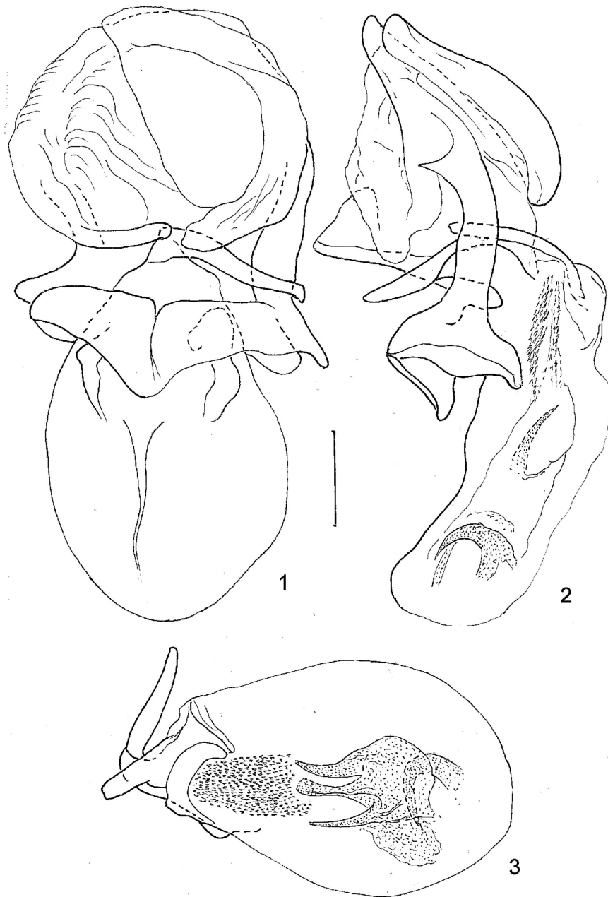
Figs 1–3. Aedeagus of Scaphisoma poussereaui sp. nov., in ventral view (1), in lateral view (2), median lobe, without parameres in dorsal view (3). Scale bar = 0.2 mm.
