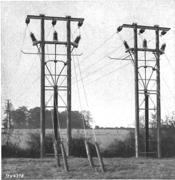
Fig. 11. «Rural Electrification». Kabelendmasten 33 kV. (Photo Henley.)
