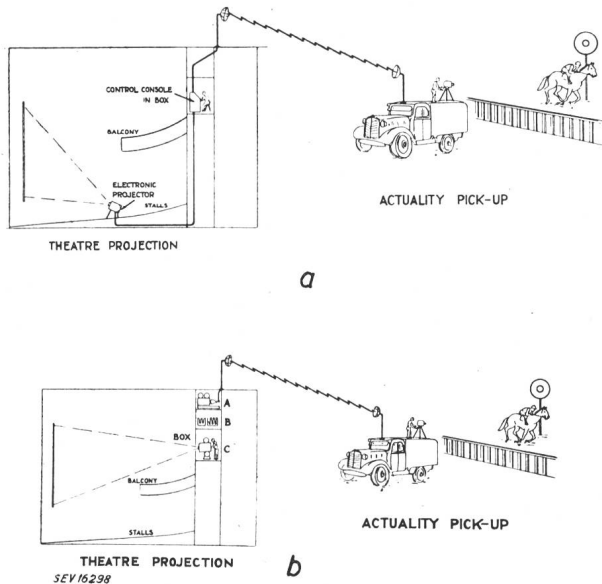
Fig. 2 a Large Screen Projection by instantaneous electronic film process b By intermediate film process Television picture recorded on film at A Film processed and dried at B Film projected by normal projector at C
