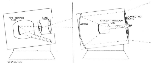
Fig. 3 Lens and Mirror Electronic Projectors
