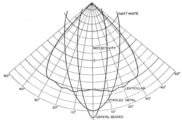
Fig. 4 Polar diagrams
