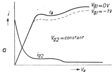
Fig. 4 a Anode and screen-grid currents of a tetrode as function of the anode voltage
