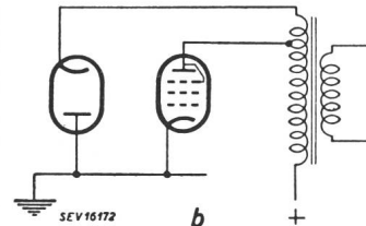
b Saw-tooth current generator with a combination of a diode and a tetrode
