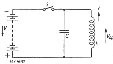
Fig. 1 Ideal circuit for generating linear saw-tooth currents in a coil
