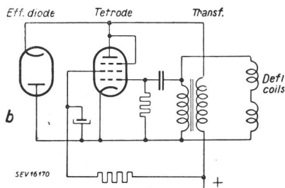
b Saw-tooth current generator with a combination of a diode and a tetrode
