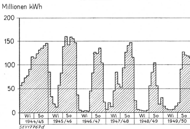
d) Elektrokessel
