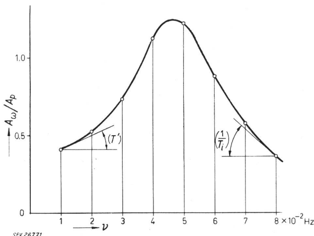
Fig. 5 Transmittance \frac{A_w}{A_p} = f(\nu)
